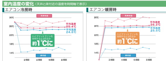
HYBRID-FAN
